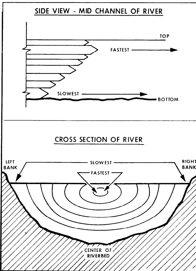
Figure 23-12. Laminar Flow.
