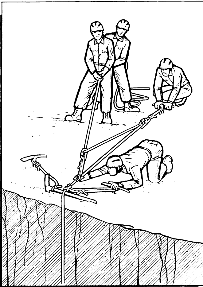
Figure 22-96. Two-Pulley System.
