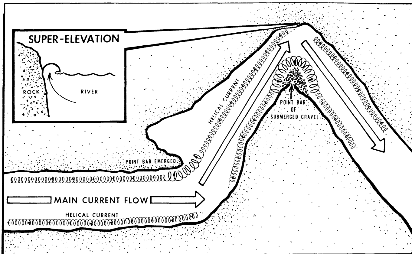
Figure 23-14. Macroturbulence.
