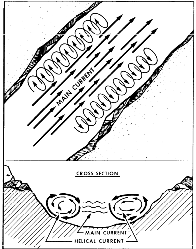
Figure 23-13. Helical Flow.
