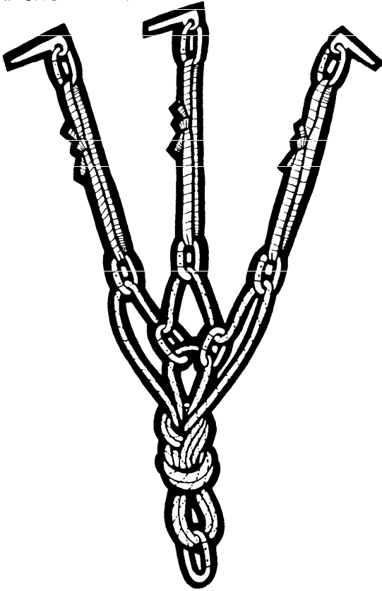
Figure 22-38. Equalizing Anchor.
